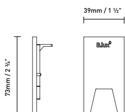
4.a. Anvil System Surface End Cap
