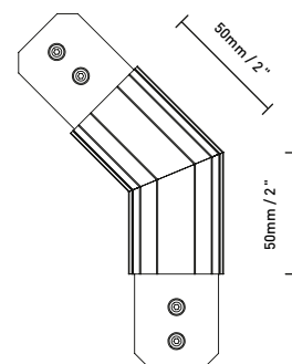
Anvil System 135° Angle
